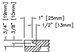
PICKHOLE DETAIL QUARTER SCALE
